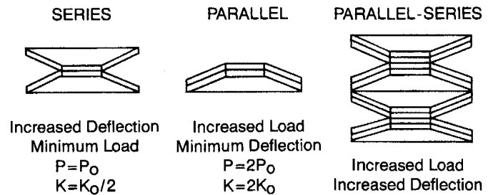
Fig. 13. Load and deflection relationships for conical spring washers stacked in series, parallel, and parallel-series combinations.
