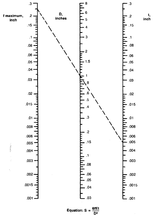
Fig. 3. Stress nomograph based on the design equations for cylindrically curved spring washers, a maximum stress of 200,000 psi, and high-carbon steel material.
