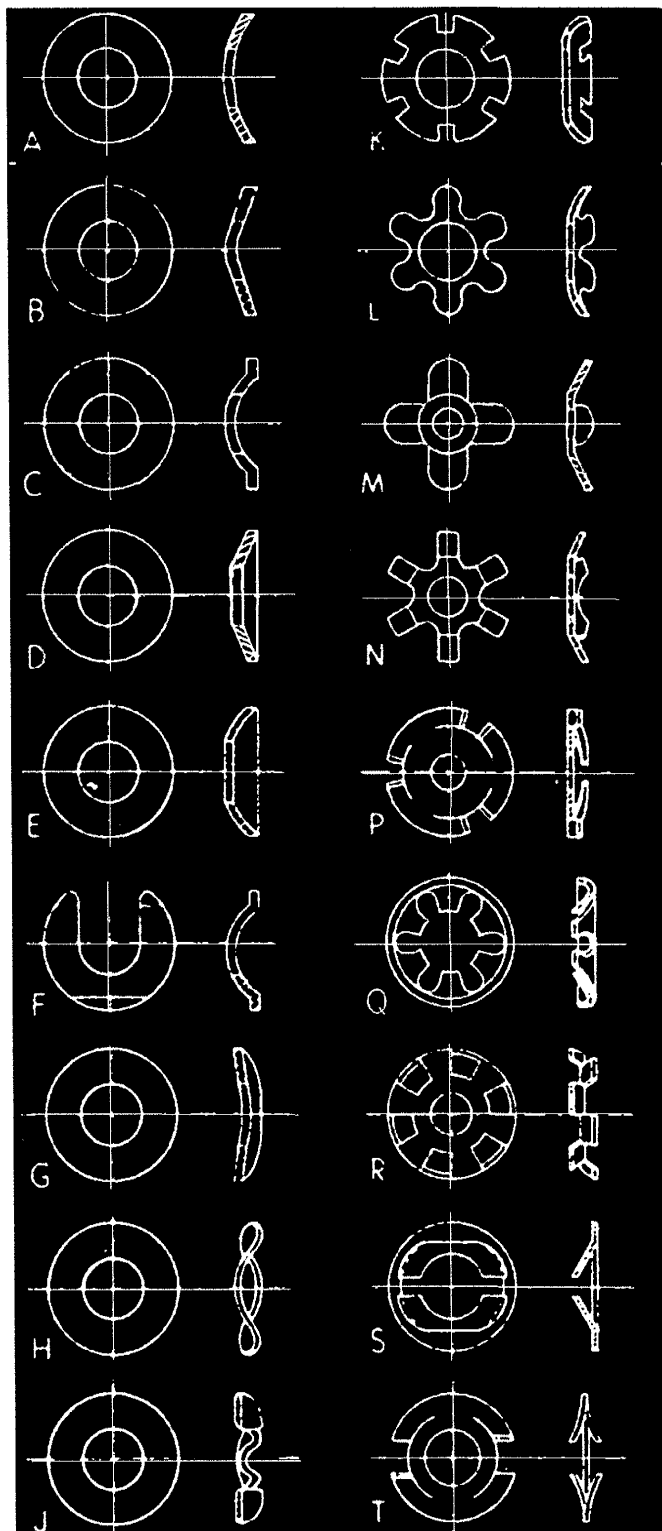
Fig. 16. Typical designs of spring washers showing the basic cylindrically curved, wave, and conical-disc types, with some of the varieties that have been developed from them.
