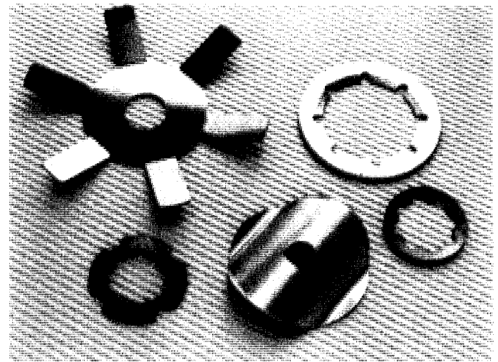
Fig. 15. Special spring washers such as these are used to provide greater deflection, special load deflection characteristics, special contact requirements, or additional functions.
