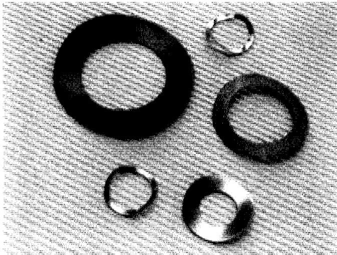
Fig. 1. Cylindrically Curved Spring washers are used where flexibility is important and loads are light. Maximum height should be less than one-half of the outside diameter.
